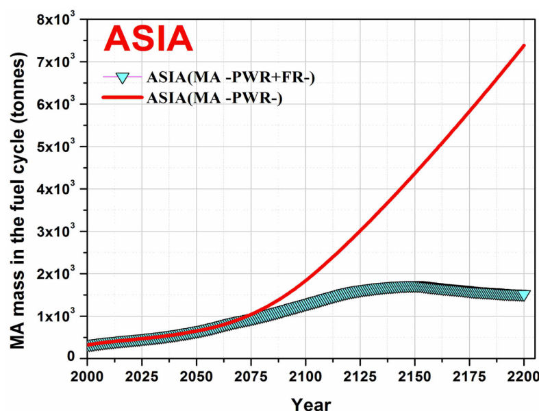
Figure 18. Comparison of the Minor Actinides (Np+ Am+Cm) inventory between the once-through (option 1, i.e. , only PWRs are deployed) and the closed fuel cycle option (option 2: FRs installed as soon as possible according to plutonium availability) in the ASIA region.
