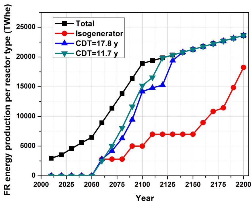
Figure 8. Nuclear energy production of fast reactor fleet.
