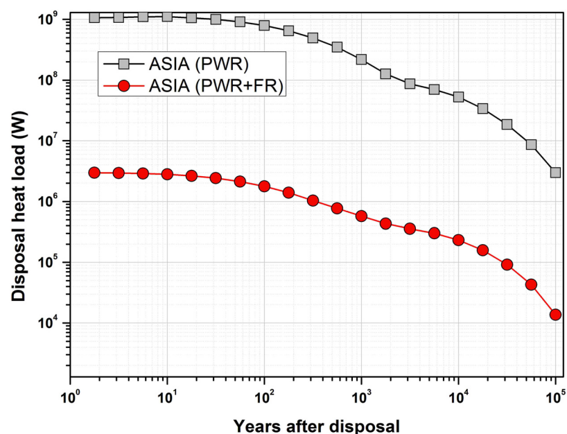
Figure 20. Comparison of the heat load in a geological disposal for the ASIA region between the once-through and the close fuel cycle options (only the MA component is displayed).
