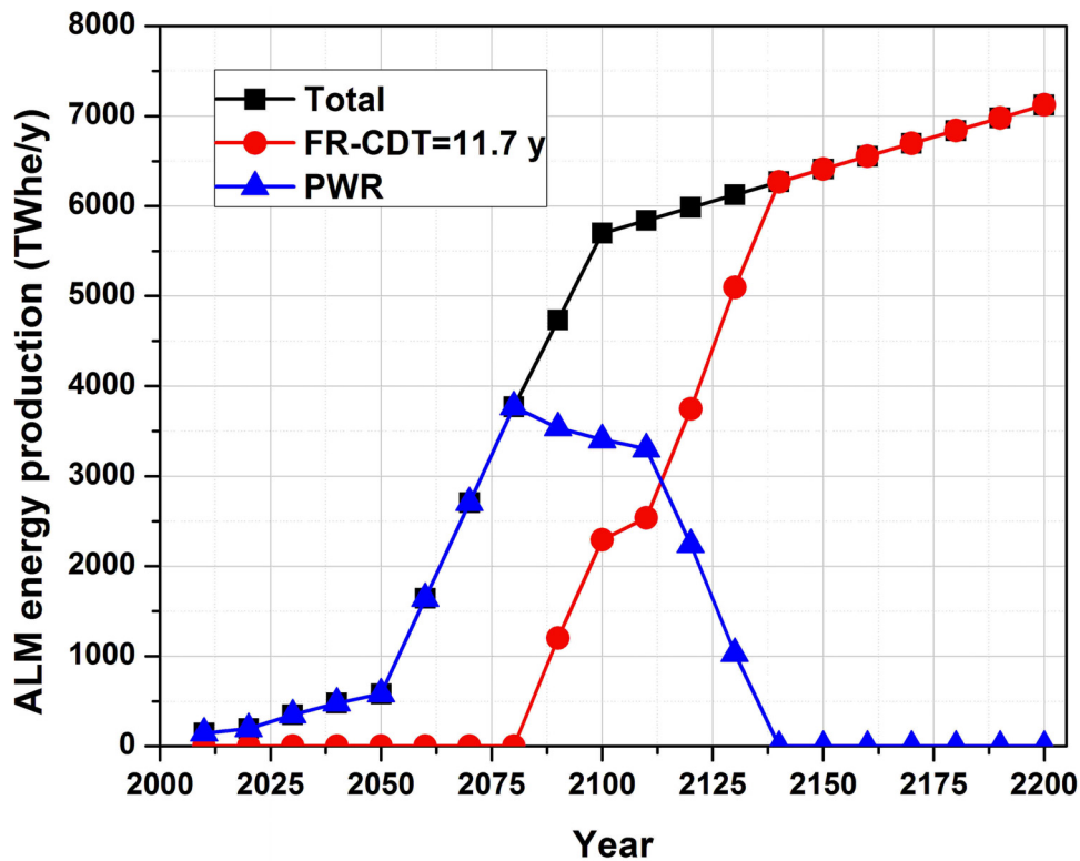
Figure 14. Nuclear energy production share in ALM (PWRs and breeders).
