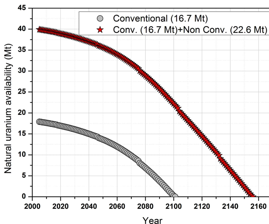
Figure 4. Natural uranium availability vs. time for pressurized water reactors (PWRs) once-through case.
