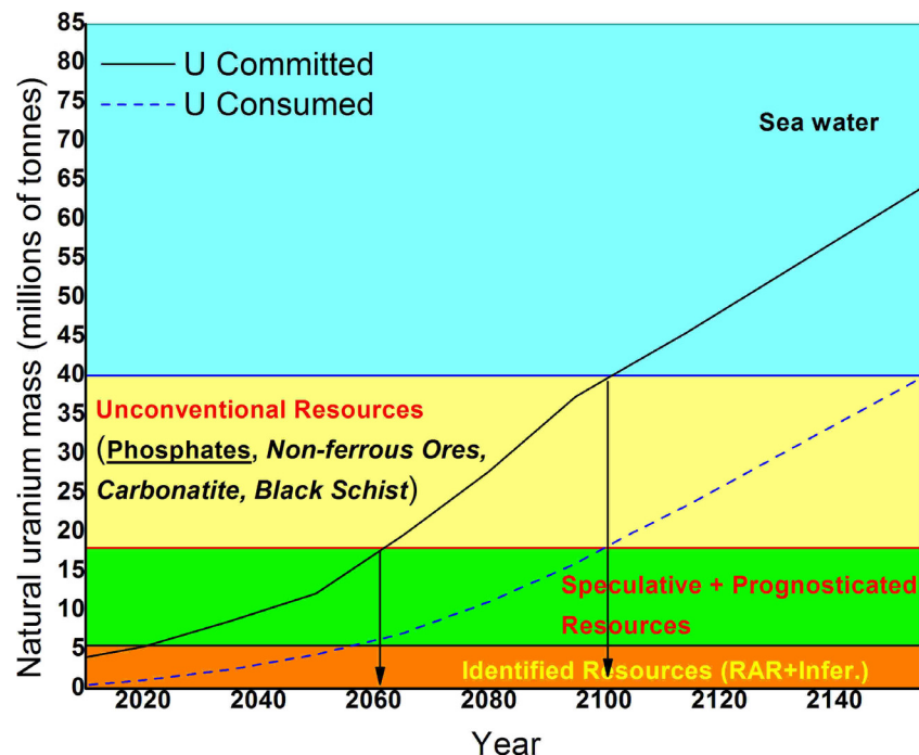
Figure 5. Natural uranium consumed and engaged for PWRs once-through case.
