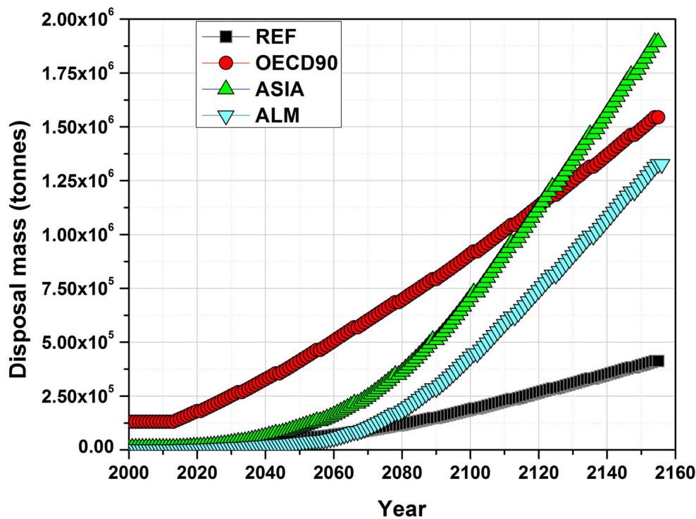
Figure 12. Spent fuel mass inventories per region (case: only PWRs deployed).
