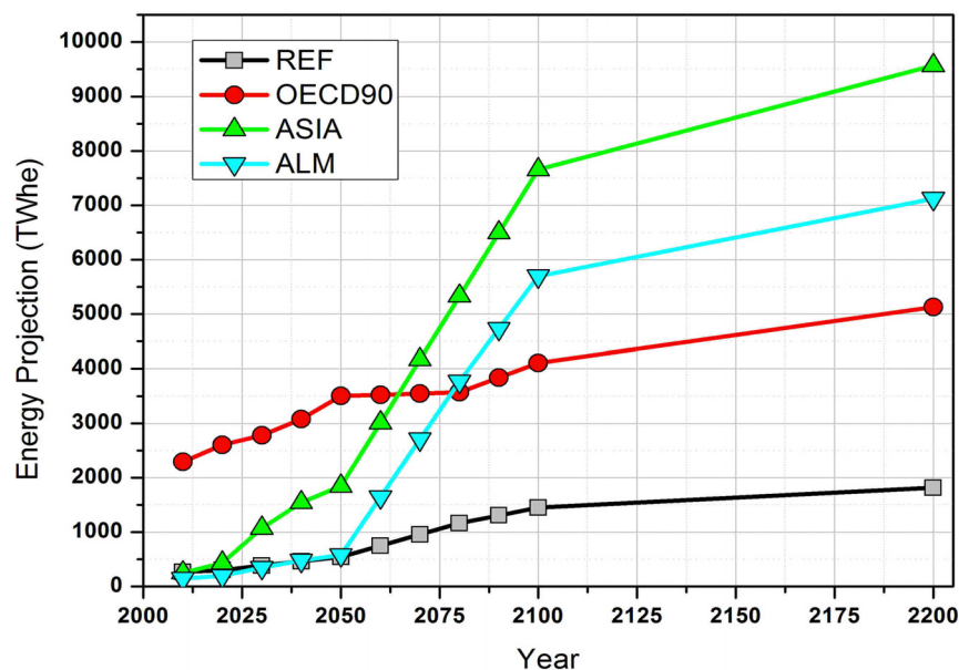
Figure 3. Nuclear Energy Projections (TWh e ) per region. B-IIASA subdivision [13] rescaled to the reference scenario total value, derived from [12], see text.
