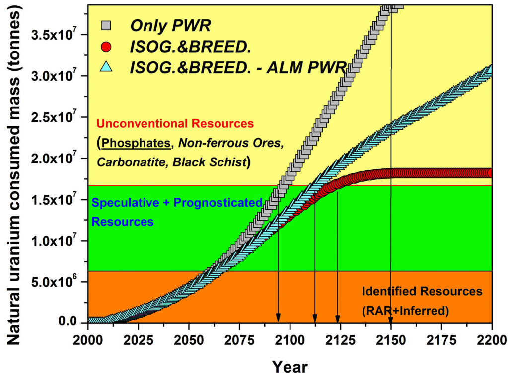
Figure 17. Total natural uranium consumptions for three different deployment scenarios ( PWRs lifetime 60 years assumed ): (■) Fuel Cycle option 1: only PWRs with open cycle; (●) option 2: ASIA and ALM (breeders) + OECD90 and REF (isogenerators) (▲) option 3: ASIA (breeders) + OECD90 + REF (isogenerator) + ALM (only PWRs).
