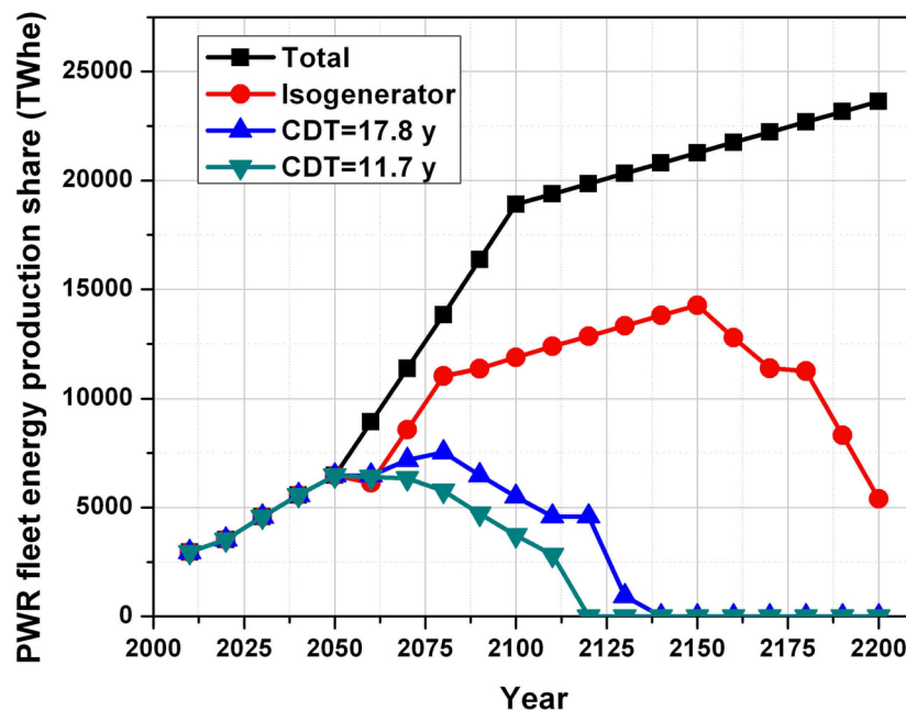
Figure 9. Nuclear energy production of supporting PWR fleet.
