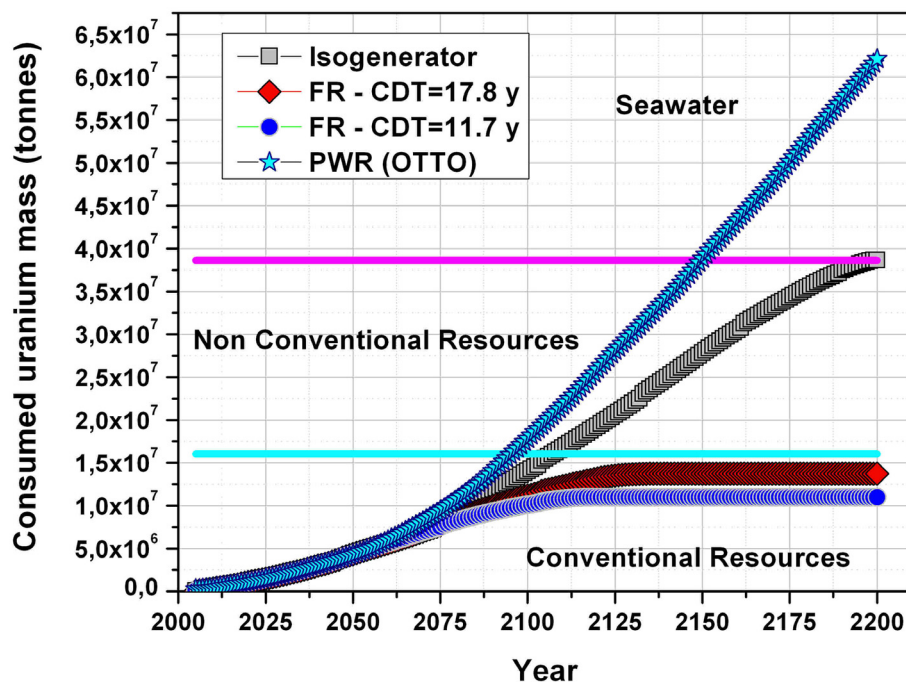
Figure 10. Mass of consumed uranium vs. time for different fast reactor classes.
