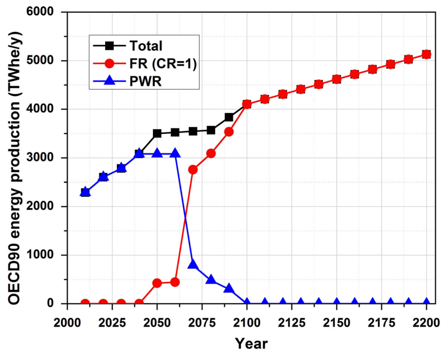
Figure 16. Nuclear energy production share in REF (PWRs and isogenerators).
