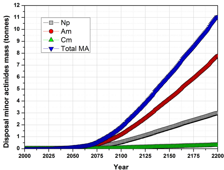
Figure 21. Total amount and share of MA to be sent to a geological disposal in the ASIA region versus time for the closed cycle option.
